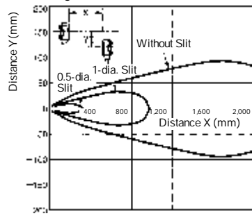
E3T-FT1j with Slit
