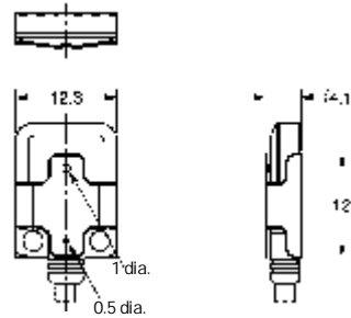
E39-S64 (for Through-beam E3T-FT1j ) With Slit mounted
