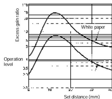
E3T-SL2j (Limited Reflective)
