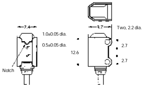
Through-beam E3T-ST1j with E39-S63 With Slit mounted
