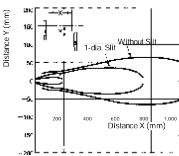
E3T-FT1j with Slit
