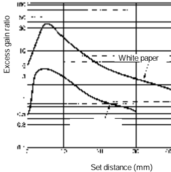
E3T-FD1j (Diffuse Reflective)
