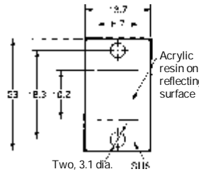
Mounting Plate
