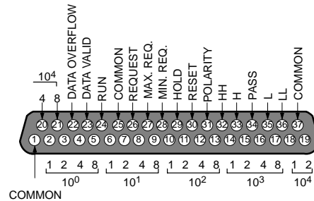
K31-B2, -B4: BCD (NPN Open Collector) (Terminals 32 to 36 are provided only on K31-B4.)
